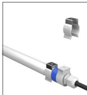
Quick-Latch Clip
